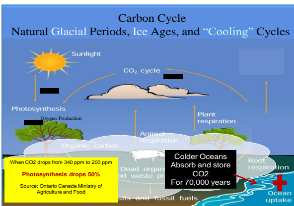
Figure 7. During winter and glacial periods ice and snow shutdowns the natural sources of carbon dioxide input into the atmosphere. When this happens, photosynthesis is likewise shutdown.
