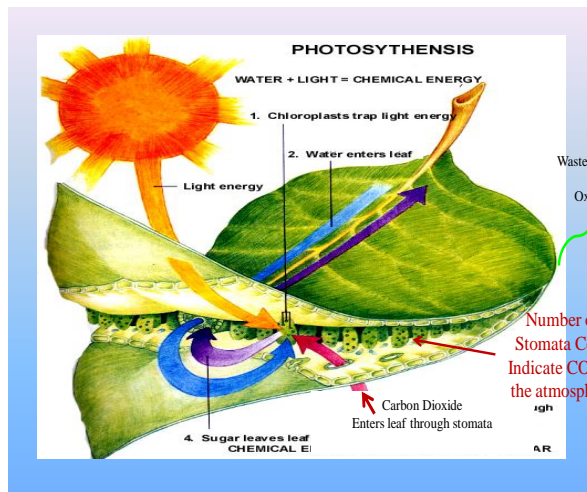
Figure 11. The plant leaf has stomata cells that take in atmospheric oxygen and carbon dioxide, then through the process of photosynthesis they release oxygen waste.
