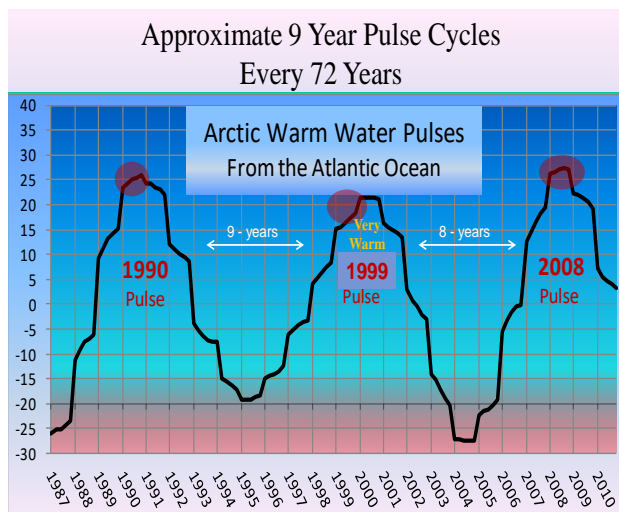
Figure 16 shows the approximate 9-year Lunisolar gravitational cycle. It is this cycle that is a major contributor to earth's climate cycles.
