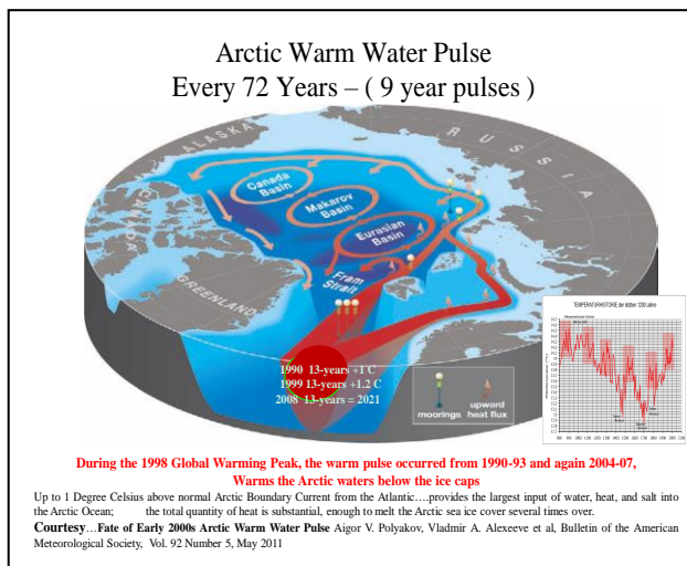
Figure 17 shows the North Atlantic warm water pulse that enters the Arctic Ocean in coincidence with the 9-year Lunisolar Pulse shown as the red dots in Figure 16.
