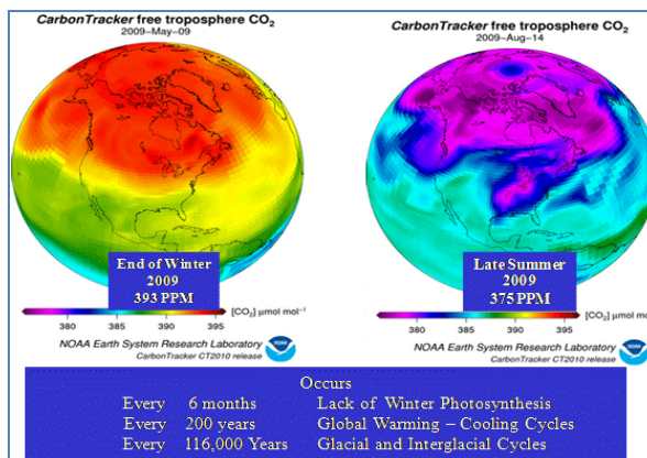
Figure 8. Left globe shows that concentrations of atmospheric carbon dioxide are much greater 6 months following the seasonal shutdown of photosynthesis. Courtesy NOAA, Climate Prediction Center carbon tracking.
