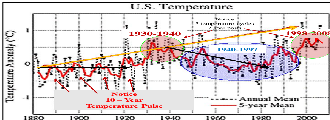
Figure 3 shows the United States temperatures in red 1880 to 2008, and the increase in carbon dioxide (orange line). Note that temperature rise and falls from 1880 to 1935 and 1940 to 1995 did not correspond to increases in carbon dioxide. Courtesy NOAA, CPC.
