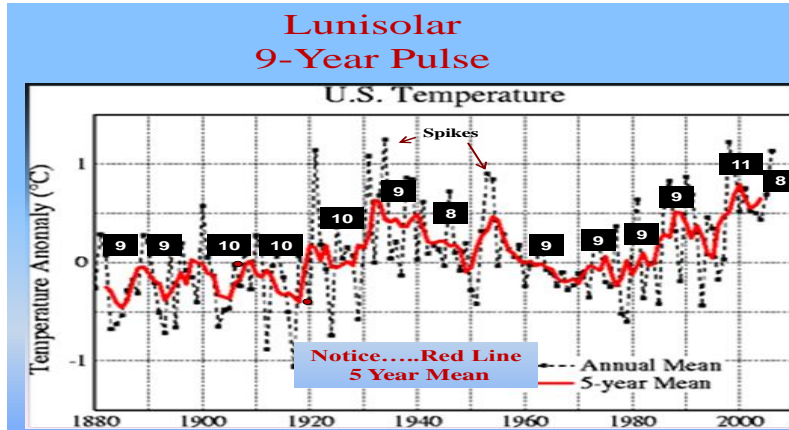
Figure 18 Shows the United States temperatures (red line) from 1880 on the left to the year 2008. Notice an approximate 9-year temperature rhythm for temperatures in the United States. Note the peaks in temperatures every 8 to 10 years, which are very similar to the 9-year Lunisolar.
